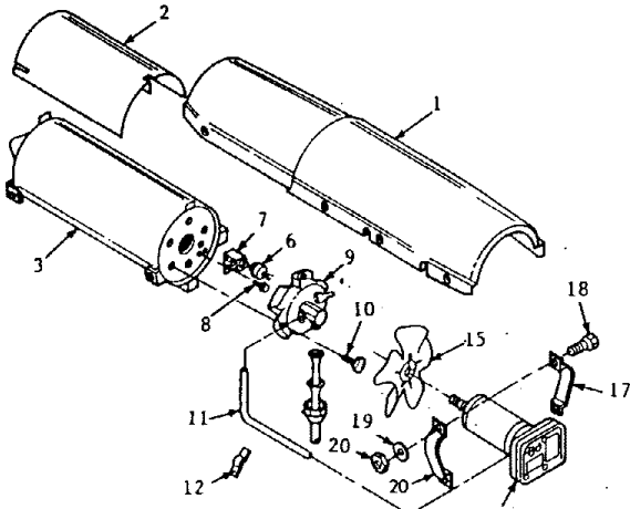
Figure 3 - Replacement Parts Illustration for Heater Model F150F
