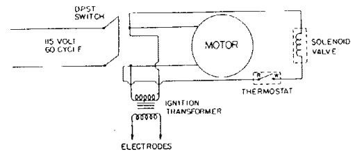
Figure 3. Diagram Thermostatically Controlled Heater
