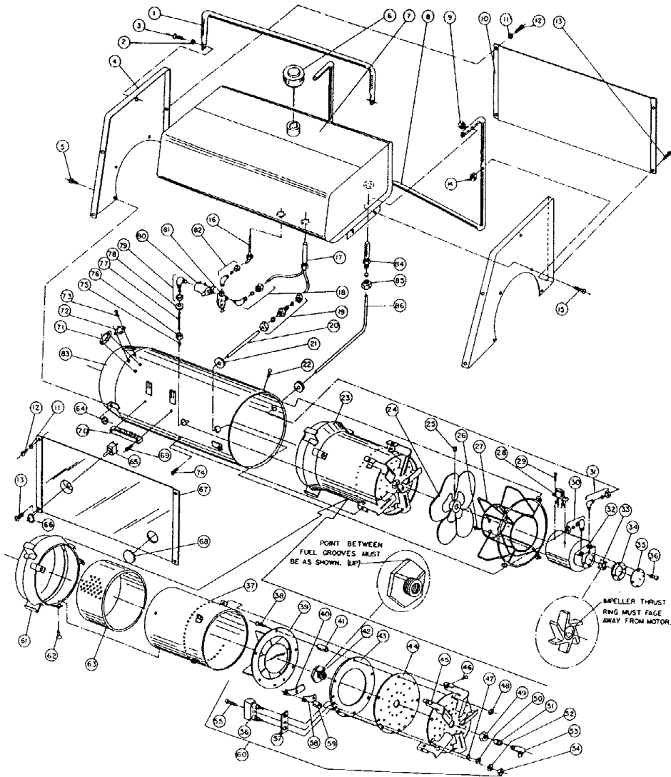
Figure 4. Exploded View
