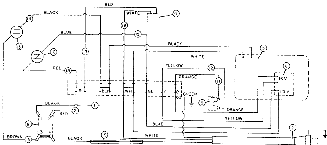
Figure 2. Wiring Diagram
