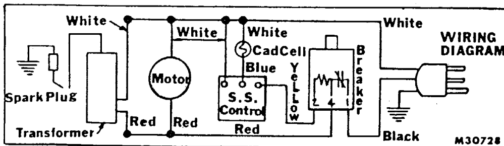
Figure 3. Wiring Diagram
