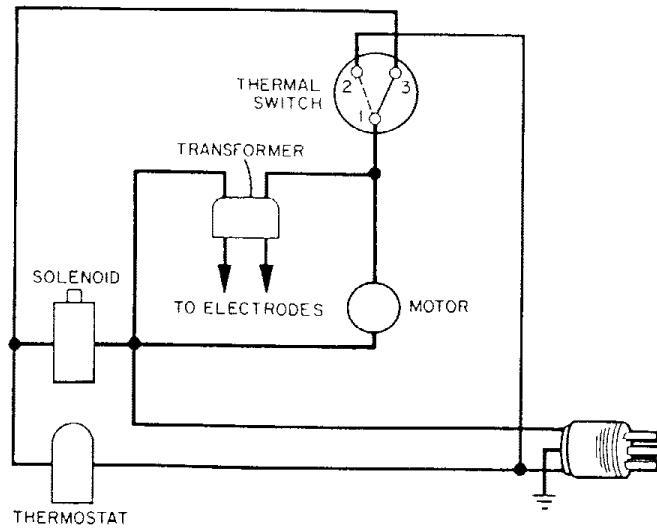
Figure 3. Wiring Diagram
