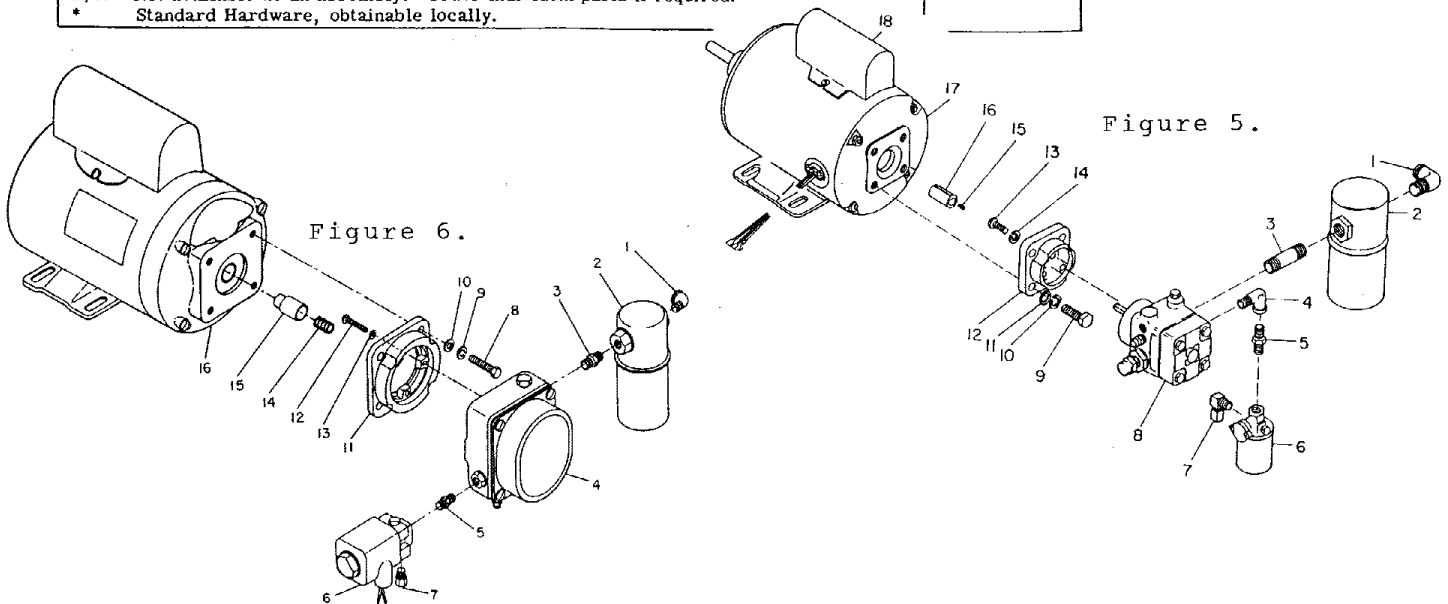
Figure 6. Motor and Pump Assembly Spec. No. 3102G02
