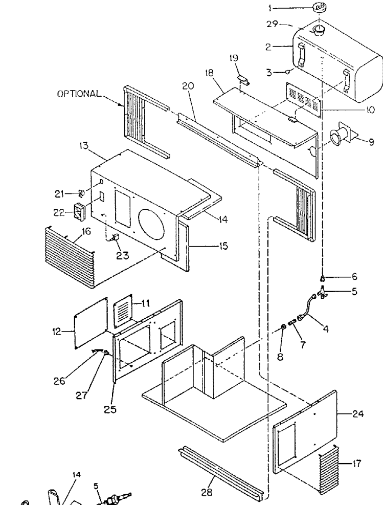
Figure 11. Tank & Covers Group
