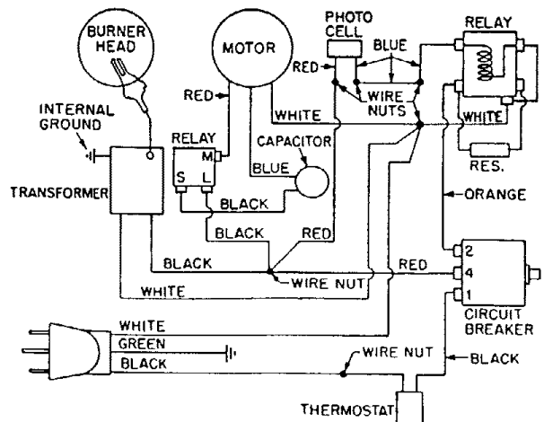
Figure 9. Wiring Diagram
