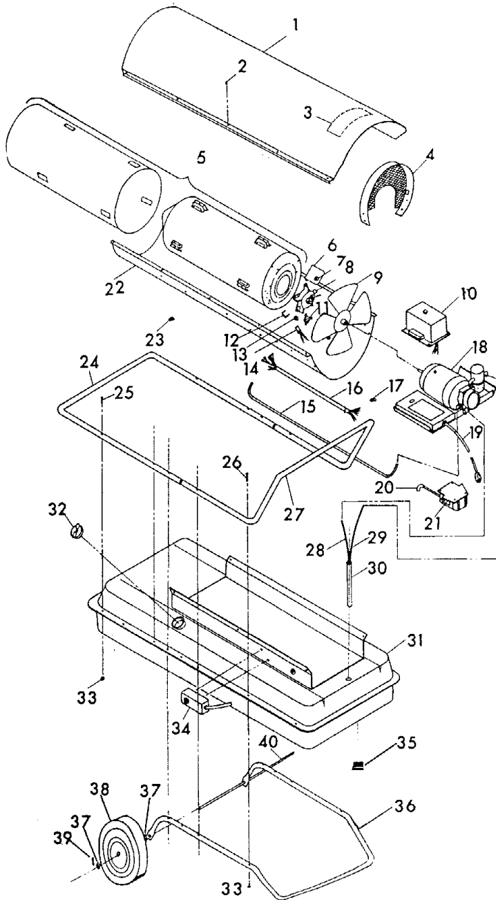
Figure 5. Heater Assembly, Exploded View
