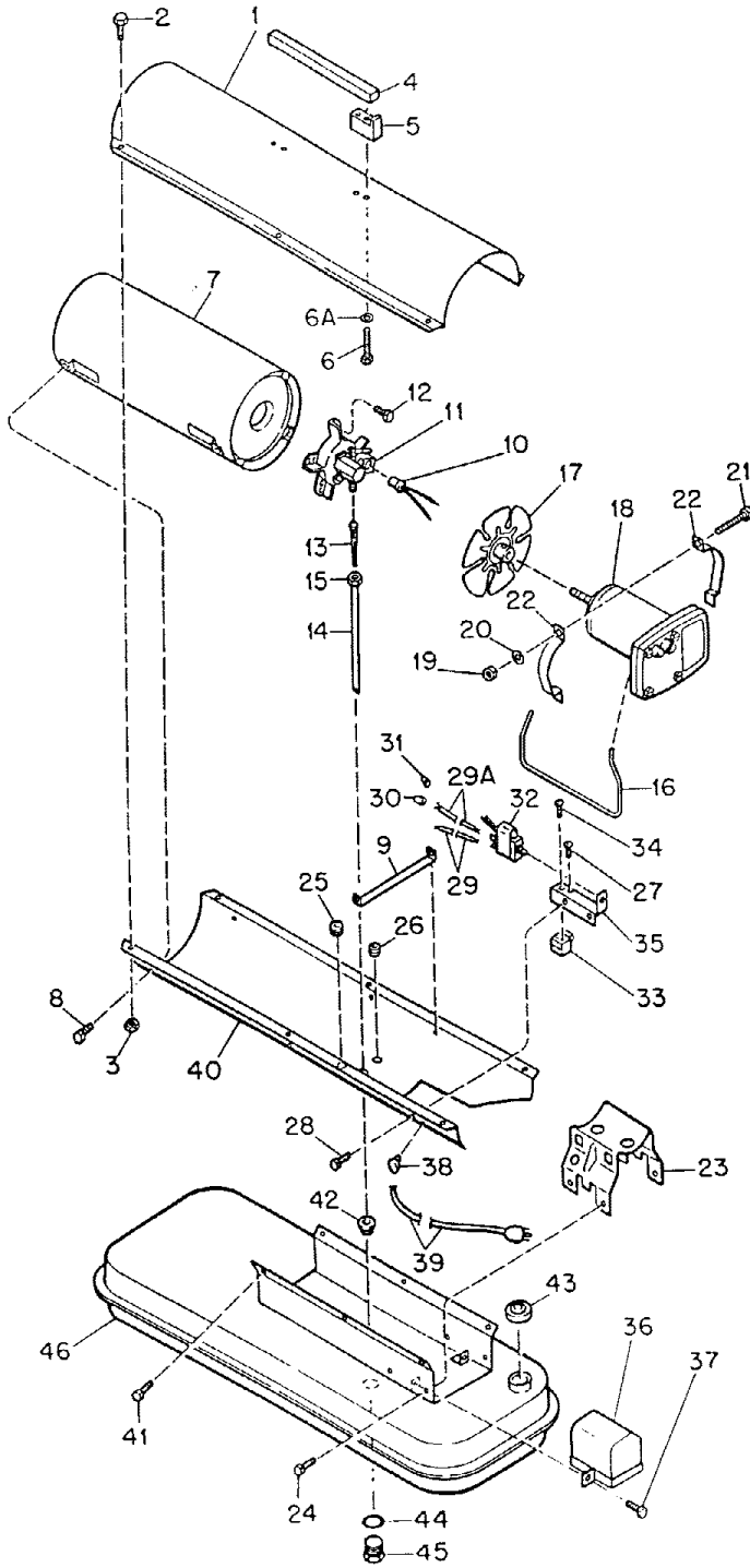
Figure 15. Heater Exploded View
