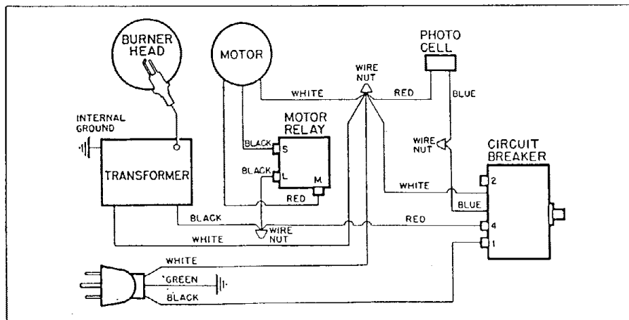
Figure 11. Wiring Diagram
